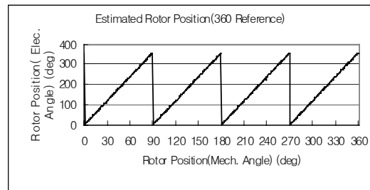
Fig. 7 Estimated rotor position
