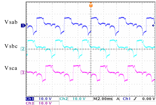
Fig. 13 Search coil's EMFs during reverse drive
