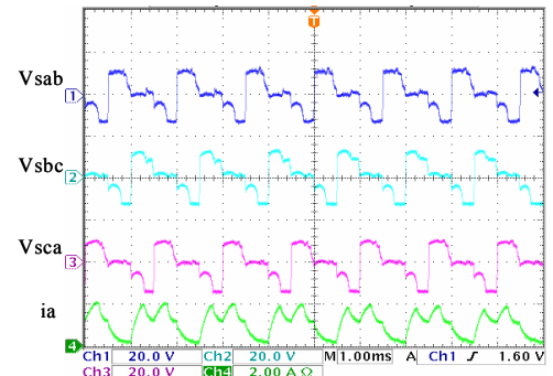
Fig. 14 Performance of the proposed method at high speed (10000rpm)
