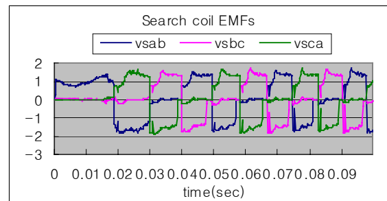
Fig. 4 Simulation waveform of search coils
