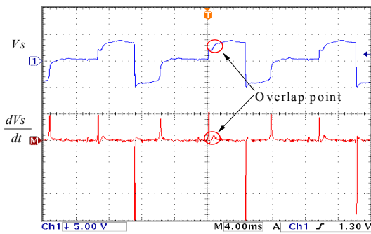
Fig. 6 Search coil's EMF and its differential waveform.
